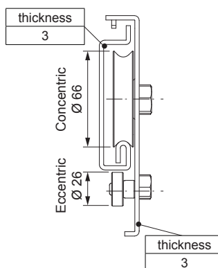
MECHANICAL DETAILS
